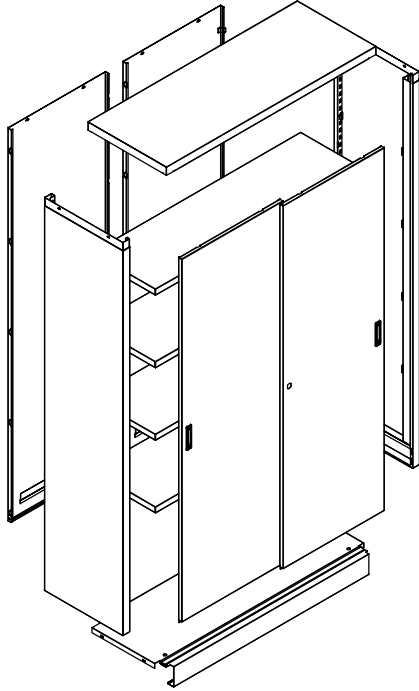
NON-ASSEMBLED VIEW
